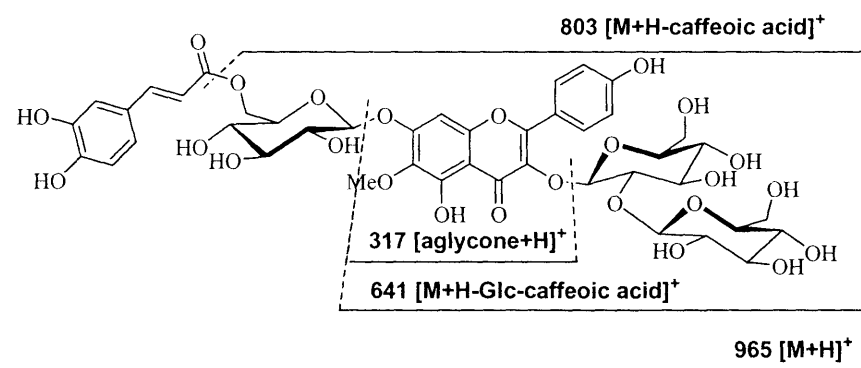
Figure 3. FAB MS/MS fragmentation pattern of 1
