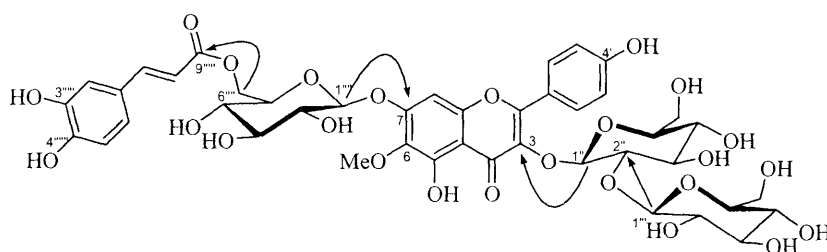
Figure 2. Key HMBC of 1 ( 1 H \rightarrow 13 C)
