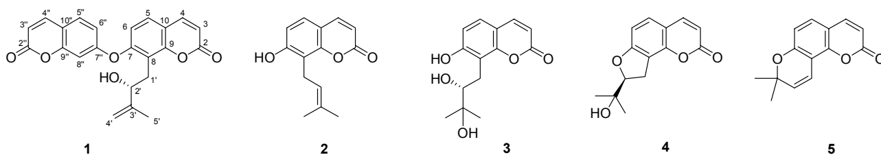
Figure 1. Structures of compounds 1-5 .
