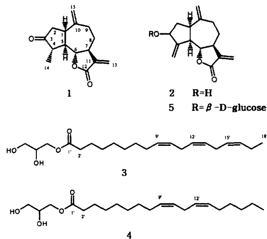
Fig. 1. Structures of compounds 1-5.
