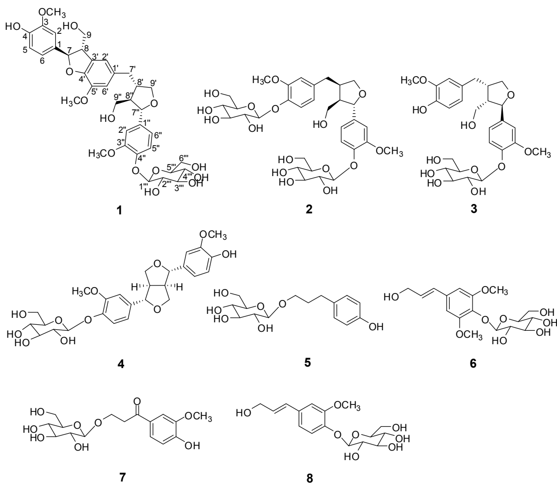
Figure 1. Chemical structures of compounds 1–8.
