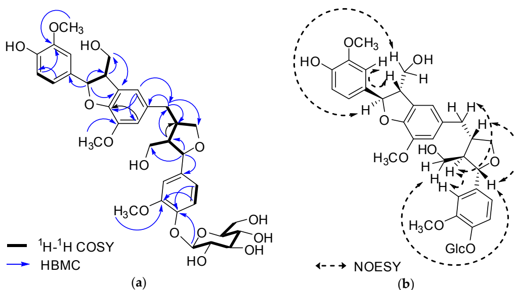
Figure 2. Key ^1\text{H} - ^1\text{H} COSY, HMBC (a) and NOESY (b) correlations of 1 .
