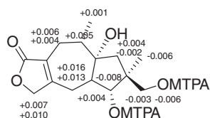
Figure 3. \Delta\delta Values ( \delta_S - \delta_R ) in ppm of the two MTPA esters derived from 1 .
