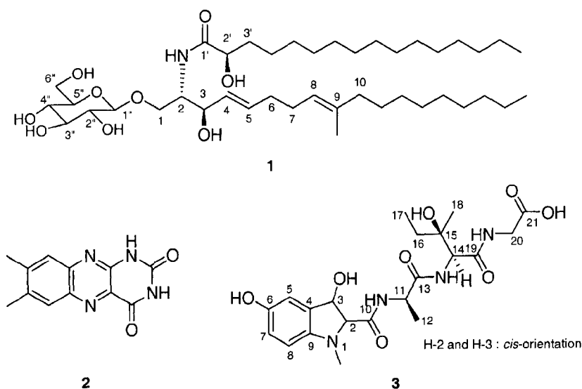
Fig. 1. Structures of compounds 1–3 from Paecilomyces sp. J300
