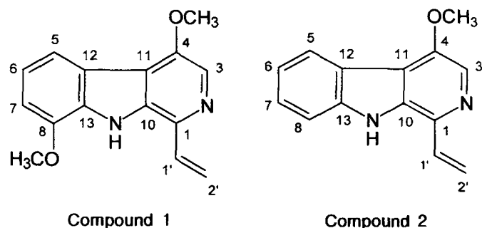
Fig. 1. Structures of compounds 1 and 2
