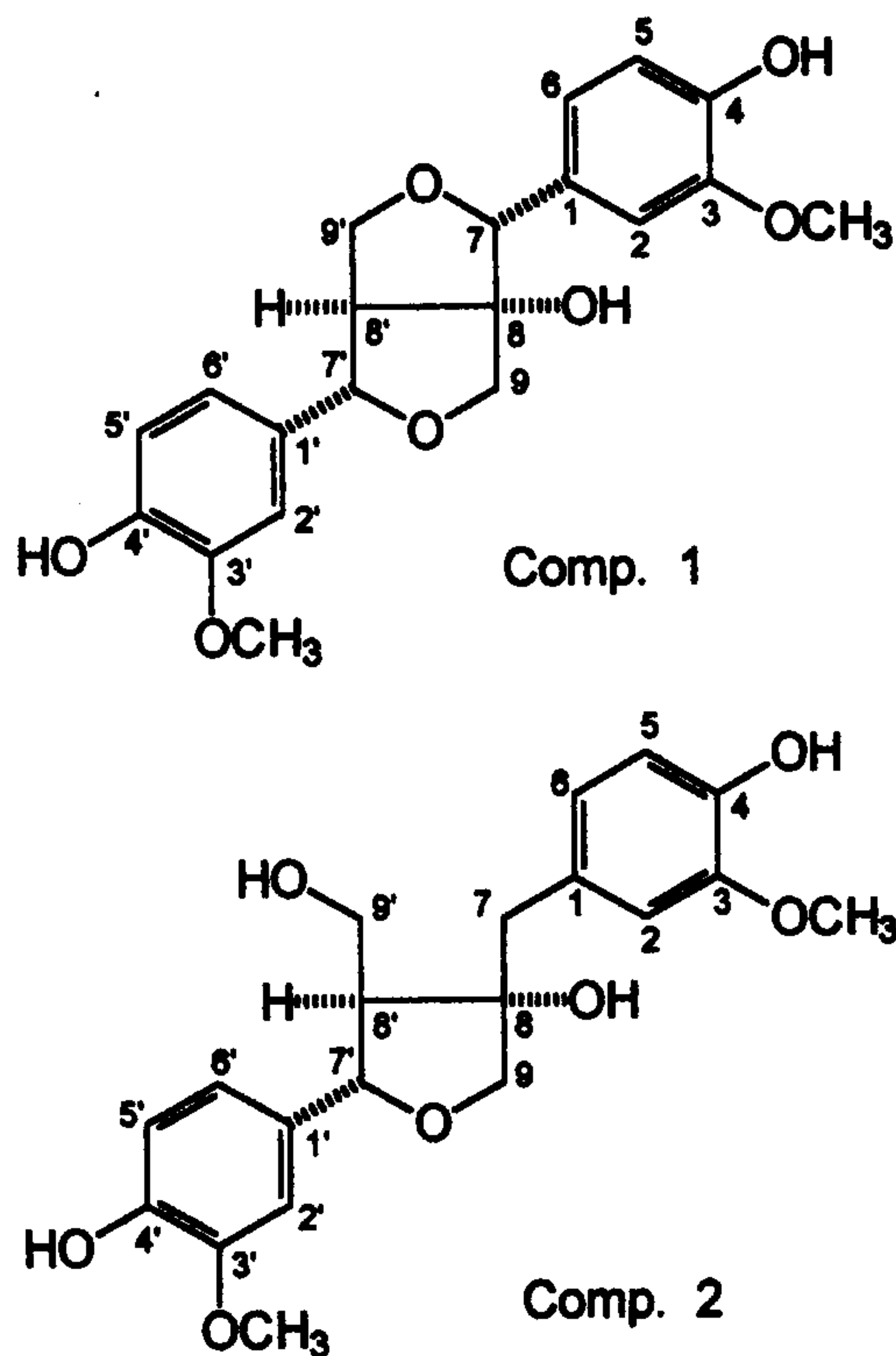
Fig. 1 - Structures of isolated lignans from Sorbaria sorbifolia var. stellipila .
