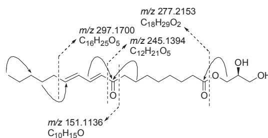
Figure 3. Key HMBC connectivities and HREIMS fragmentation of 1 .
