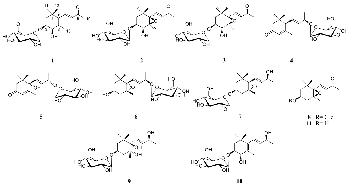
Fig. 1. The Structures of the Isolated Compounds 1 – 11 from C. komarovii
