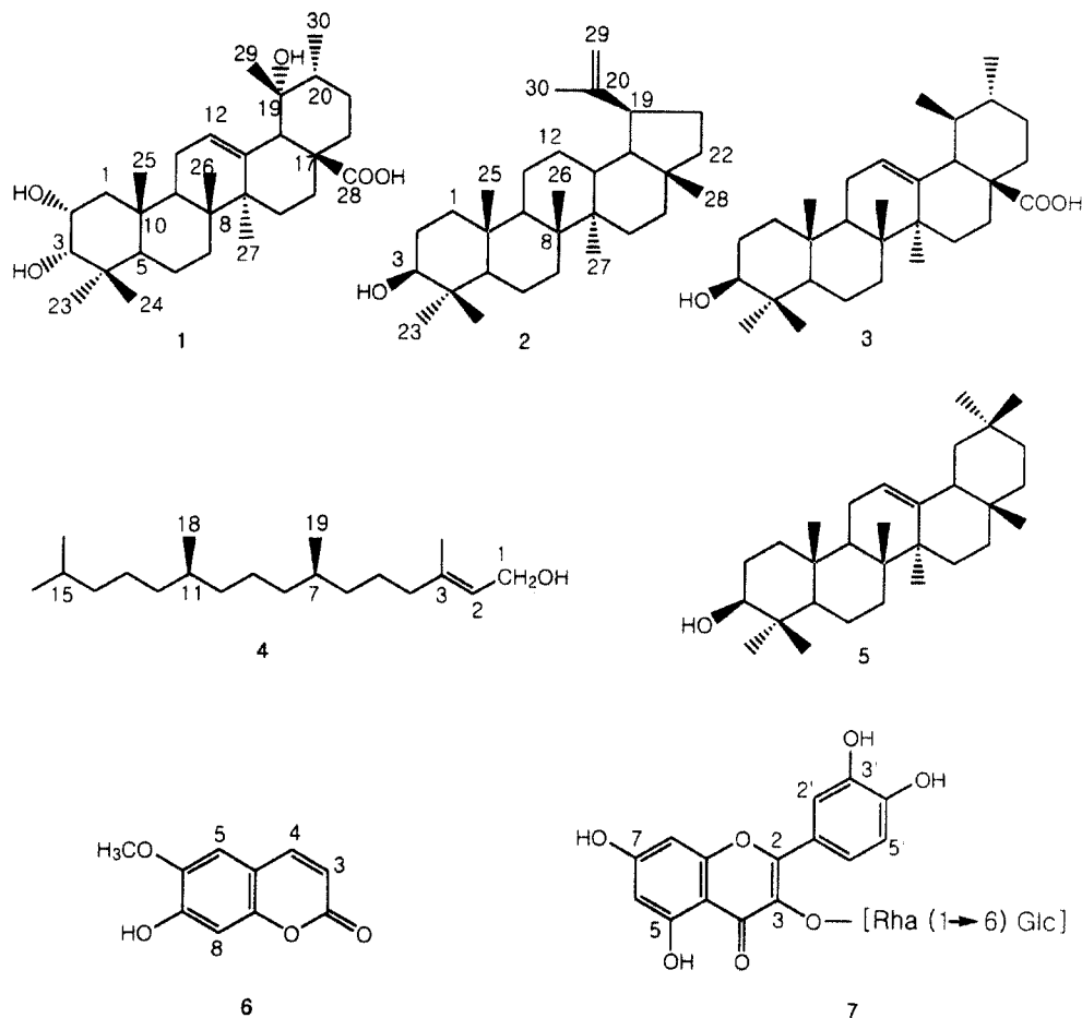
Fig. 1. Structures of compounds 1-7.
