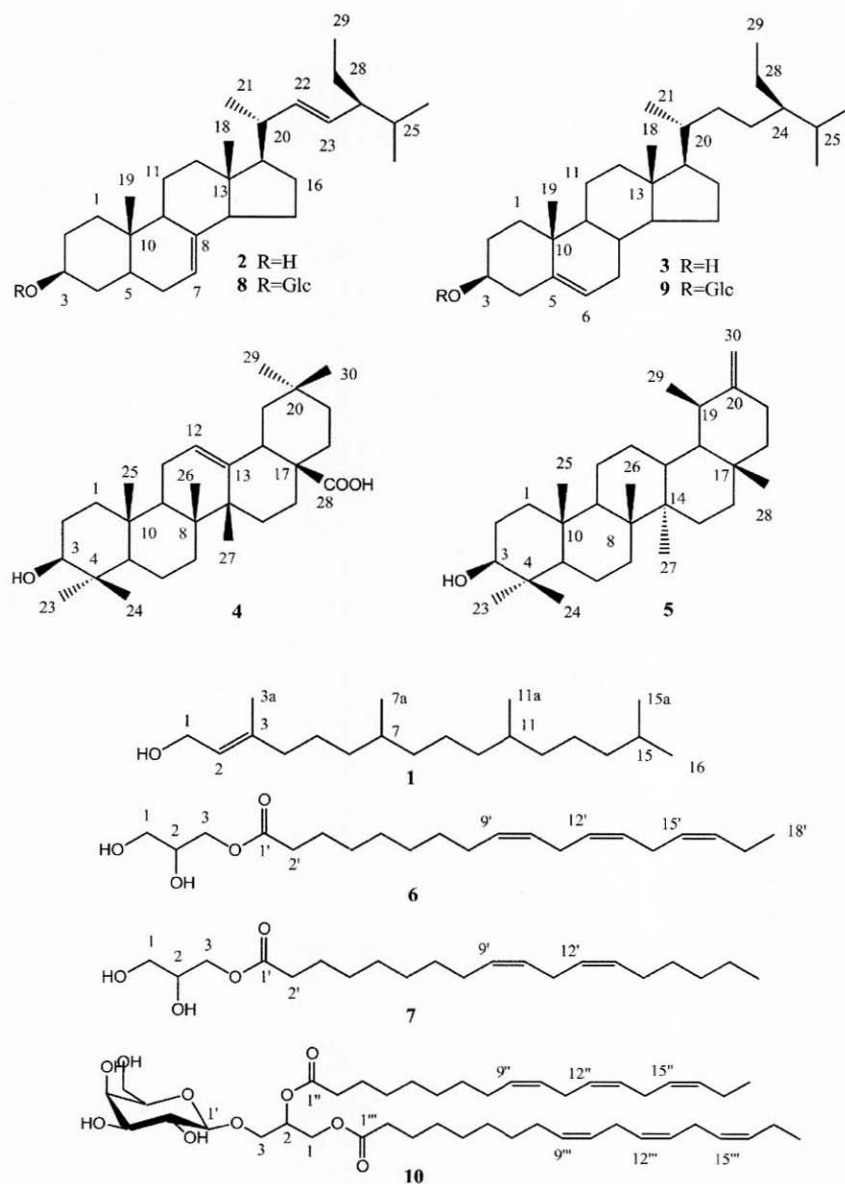
Fig. 1. Structures of compounds 1 – 10.
